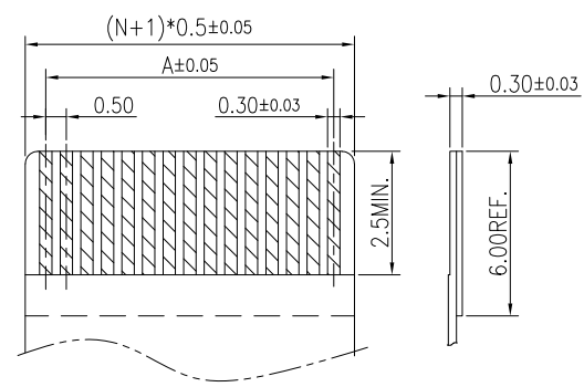
RECOMMENDED FPC/FFC DIMENSION
